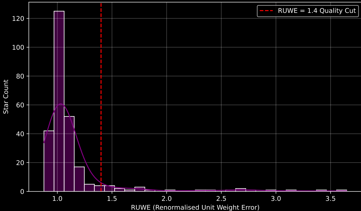
GAPOGEE DR17 Field [256+26] RUWE Distribution (n= 267)
