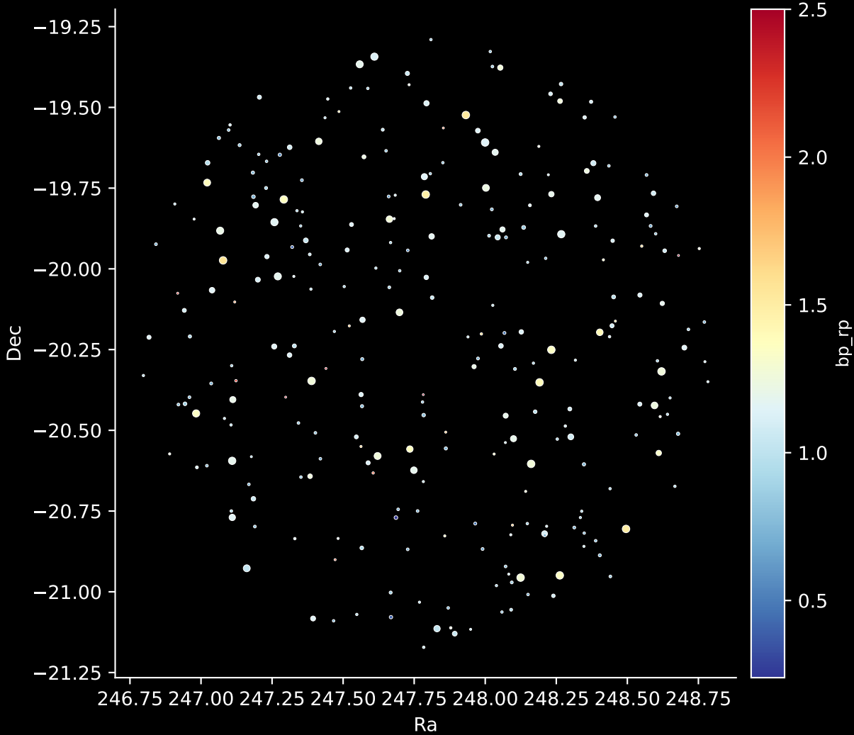
APOGEE DR17 Field: [256+26] Stars: 272
