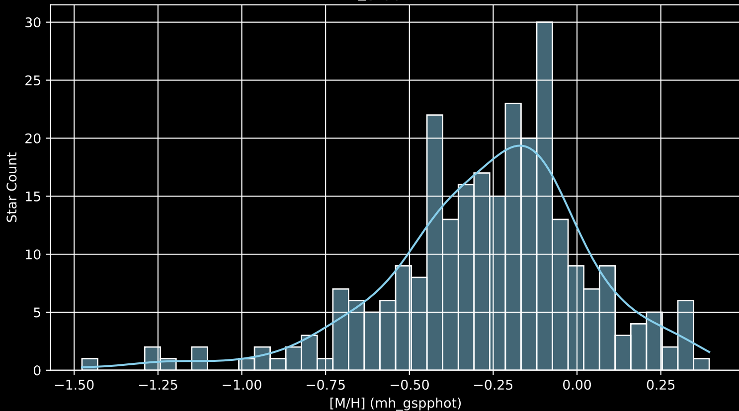
APOGEE DR17 Field: [256+26 [M/H] (mh_gspphot) (n= 272)
