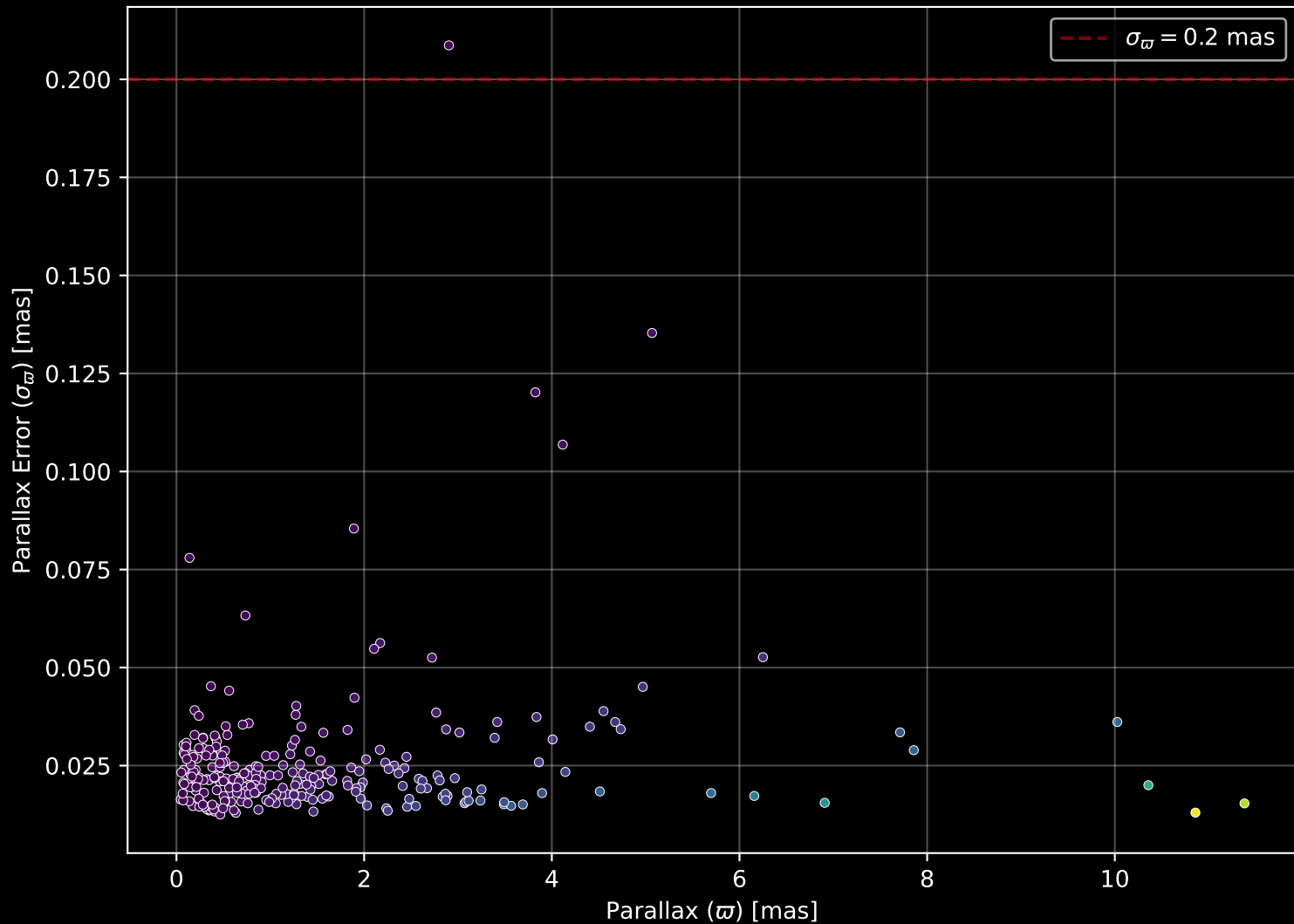
APOGEE DR17 Field: [256+26] Parallax Quality (n= 272)
