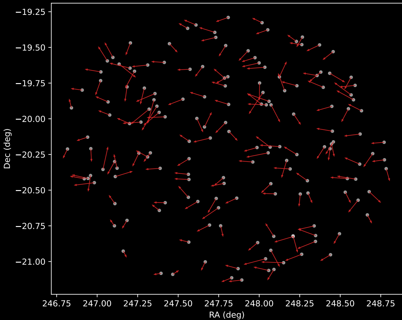
APOGEE DR17 Cluster 6 Proper Motion Vectors (n=162)
