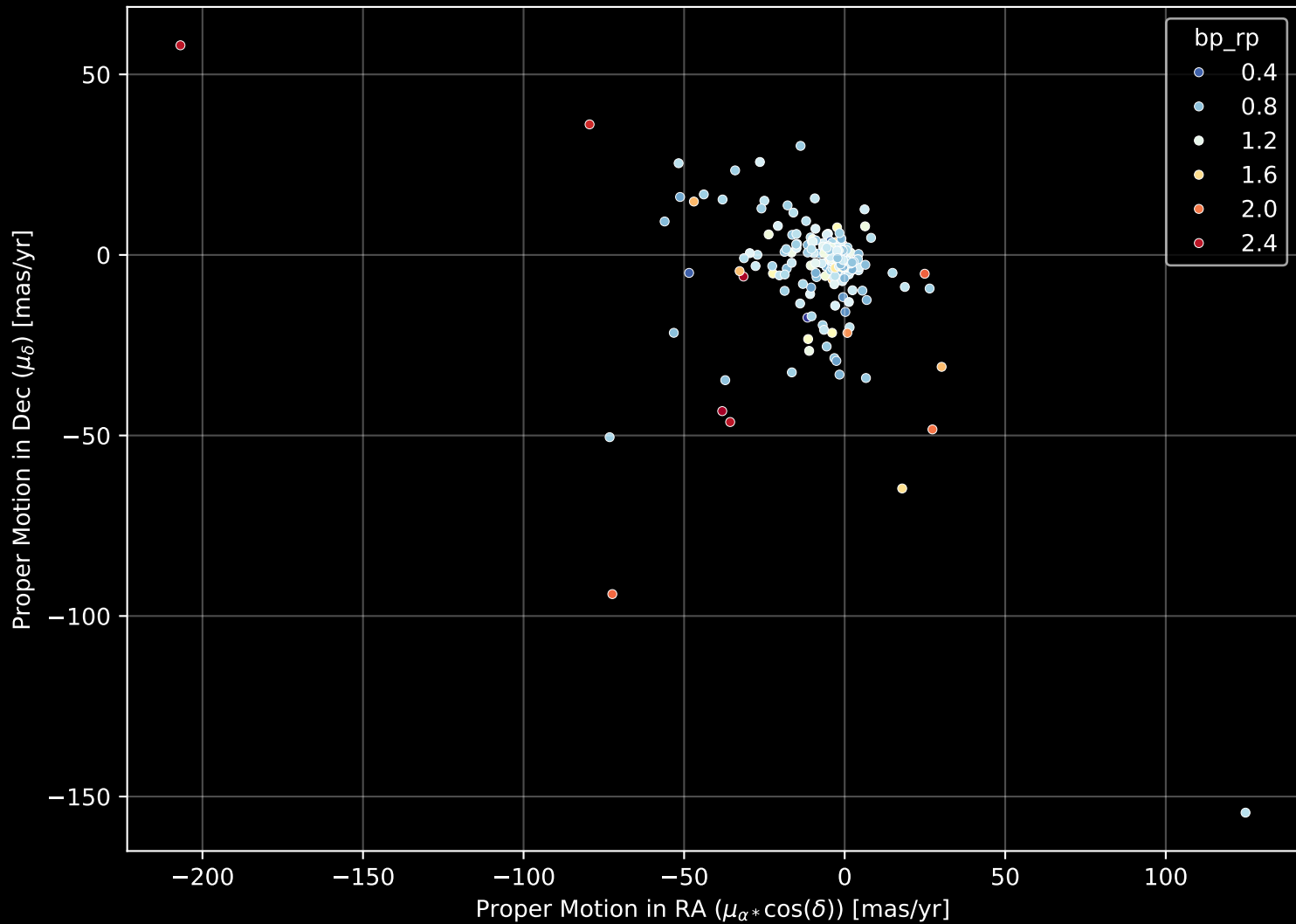
APOGEE DR17 Field: [256+26] Proper Motion Diagram (n= 272)
