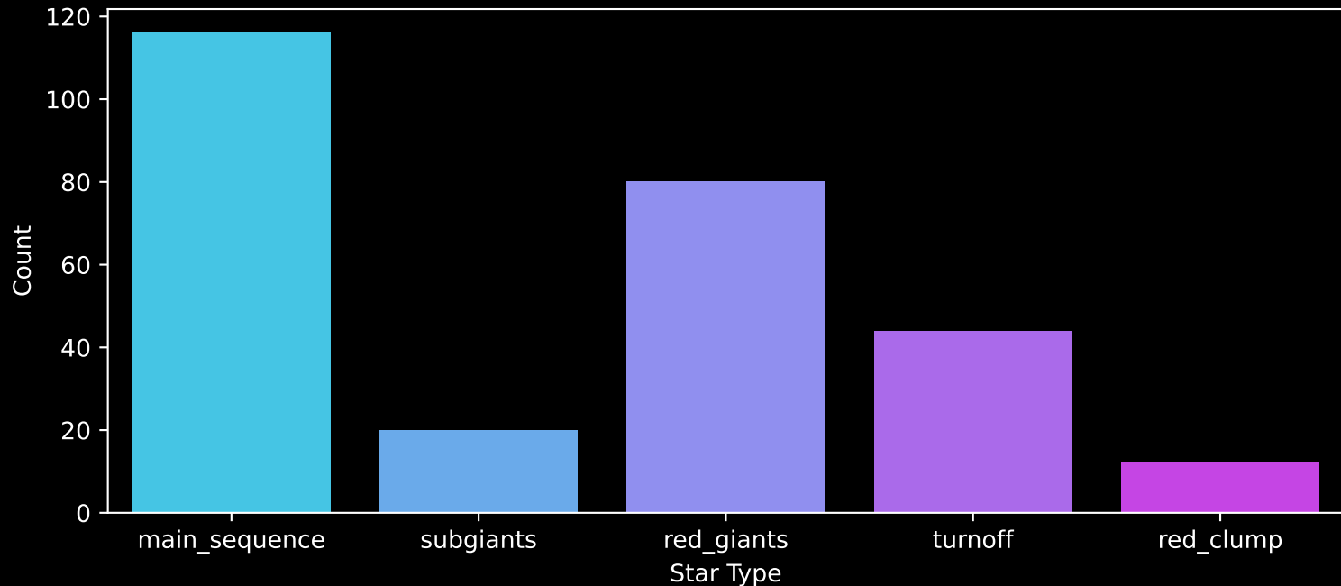
APOGEE DR17 Field: [256+26] Count plot of Star Type
